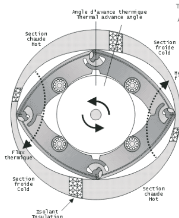
Quasiturbine Stirling Engine - Concept
