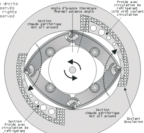
Quasiturbine Stirling Engine - Design
